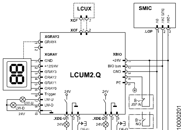
SLCU(M)2.Q connections [20023; 04.01.2007]
