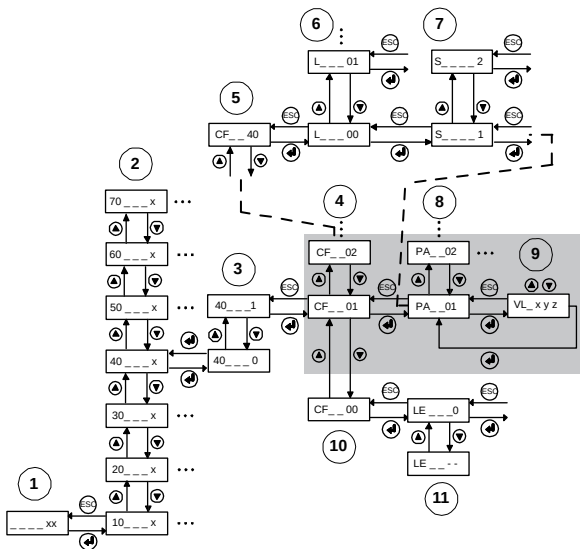
Menu Tree (6-digit display shown) [608208_010; 01.04.2016]
