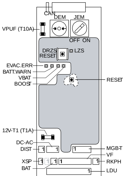
PCB Layout SEM31/32/35/36 [608208_013; 31.03.2016]
