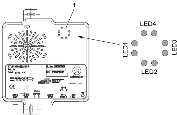
Connectivity Indication LEDs [608208_019; 08.04.2016]
