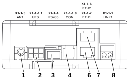
Connectors on ETMA-MR-GSM-1-* [608208_017; 07.04.2016]
