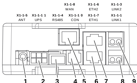
Connectors on ETMA-MR-GSM-1-* [608208_018; 07.04.2016]
